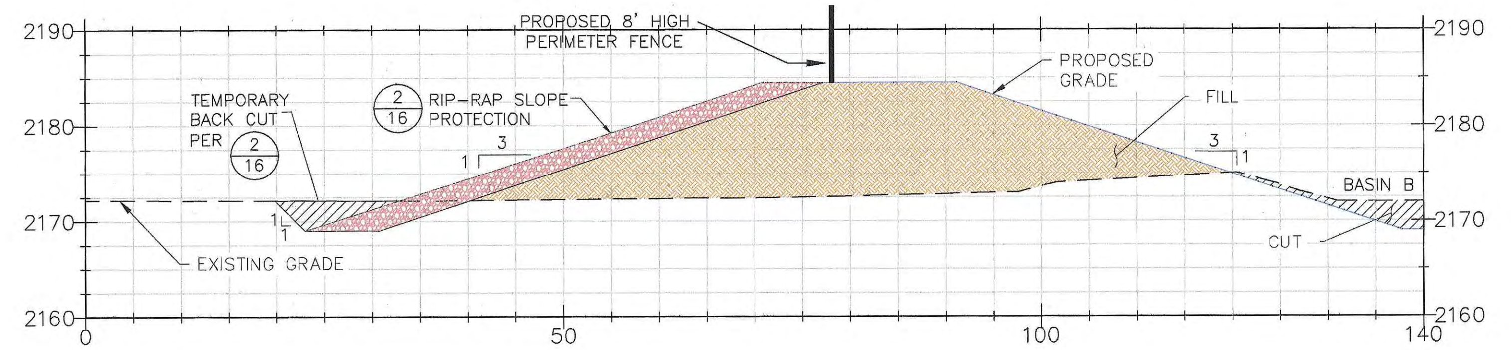
SECTION D WEST CELL SCALE: 1"=10'
