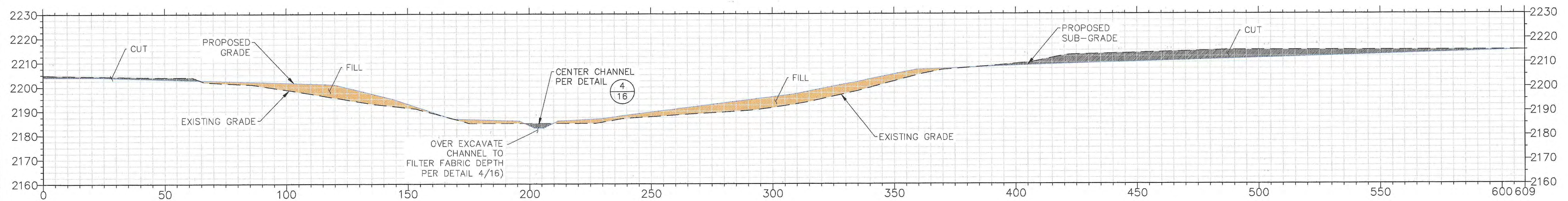
SECTION F CENTRAL CHANNEL SCALE: 1"=10'
