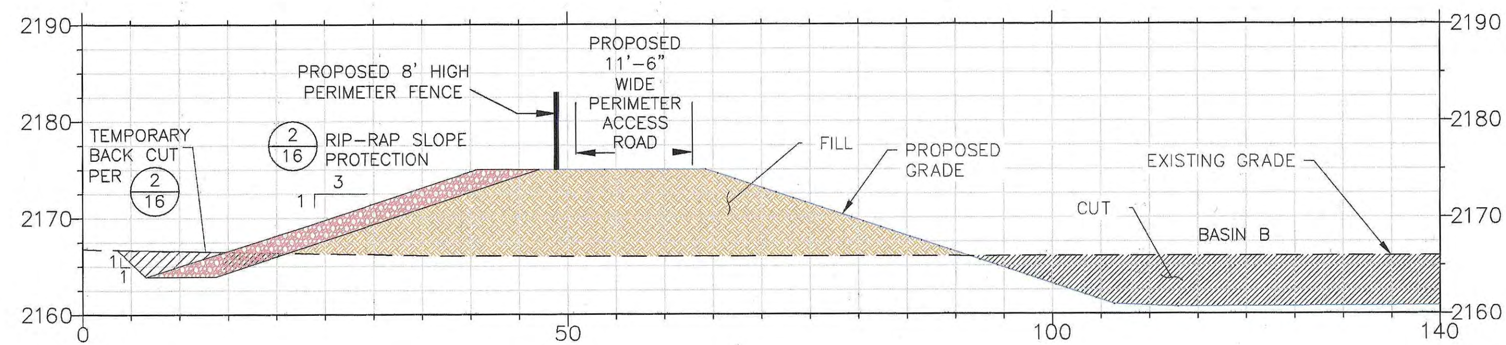
SECTION C WEST CELL SCALE: 1"=10'
