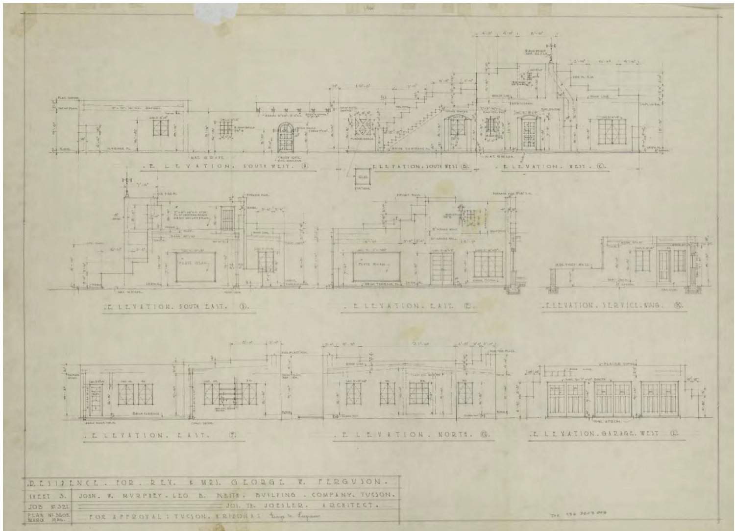
Fig. 3 Joesler Elevation Plan (Ferguson House) 1936 South, East and West elevations, Arizona Architectural Archive
