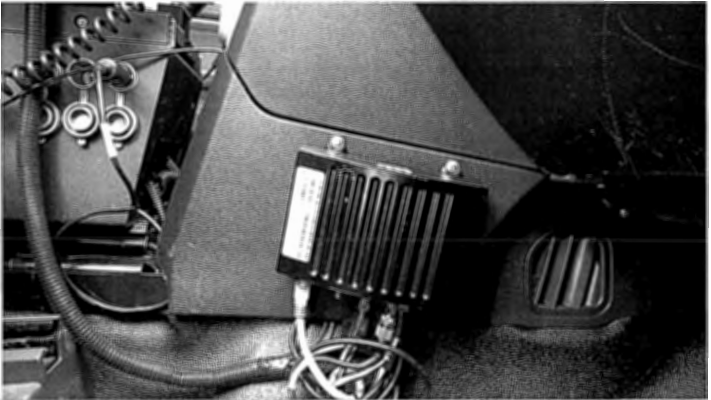
2013 Explorer Passenger Side Screw-Mounted Modem:
