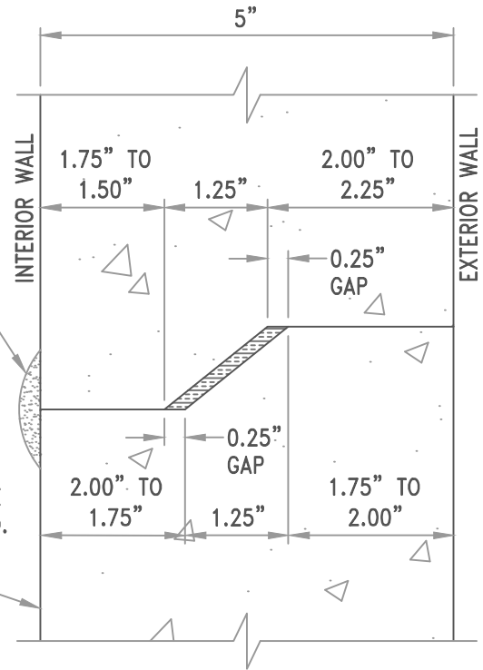
"BELL-UP" JOINT (CLOSED) N.T.S.
