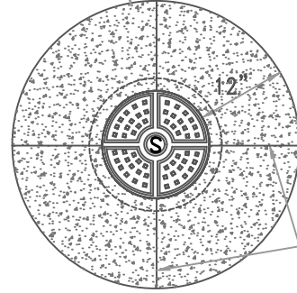
PLAN VIEW ROUND COLLAR (PAVED AREAS) N.T.S.
