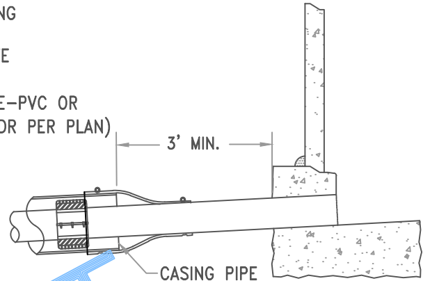
MINIMUM DISTANCE FROM MANHOLE N.T.S.
