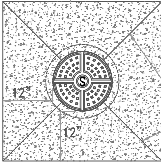
PLAN VIEW SQUARE COLLAR (UNPAVED AREAS) N.T.S.
