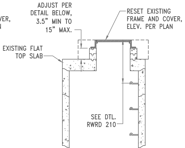
PRECAST MANHOLE WITH FLAT-TOP SLAB N.T.S.
