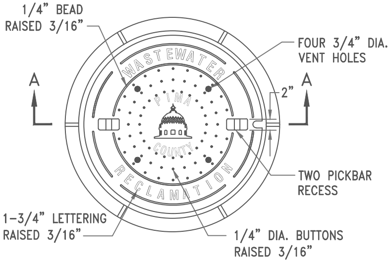
FRAME AND COVER - PLAN VIEW N.T.S.
