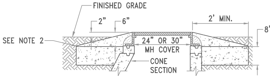
SECTION A-A (FOR CONE SECTIONS) N.T.S.
