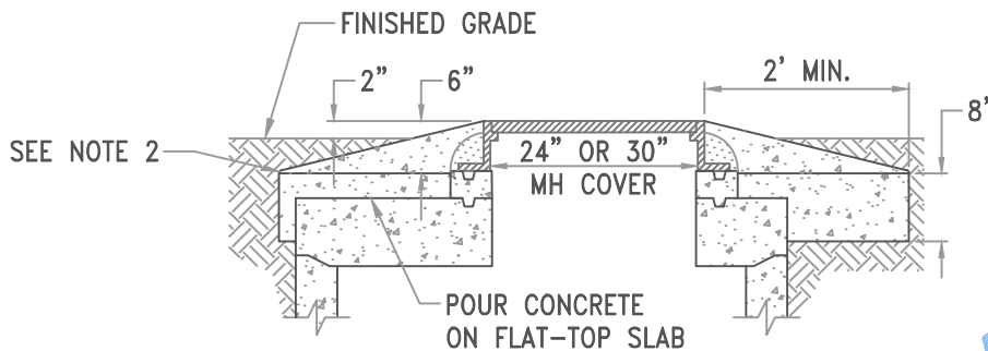
SECTION A-A (FOR FLAT-TOP SLABS) N.T.S.
