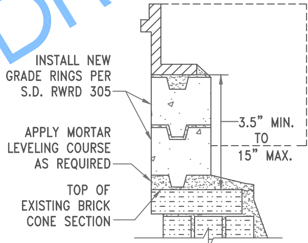
GRADE RING ADJUSTMENT N.T.S.
