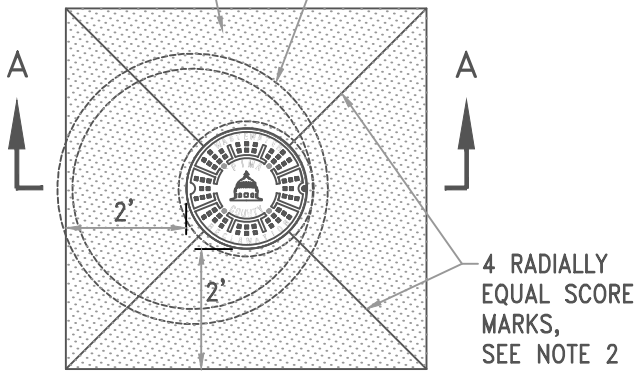
PLAN VIEW SQUARE COLLAR N.T.S.
