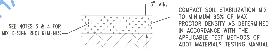
(A) STABILIZED SURFACE TREATMENT N.T.S.
