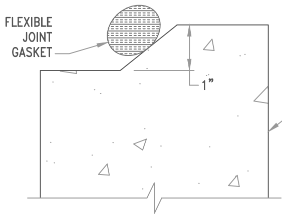
"BELL-UP" JOINT (OPEN) N.T.S.
